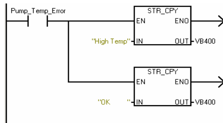
Figure 4-20 Using STR_CPY to Create Strings
