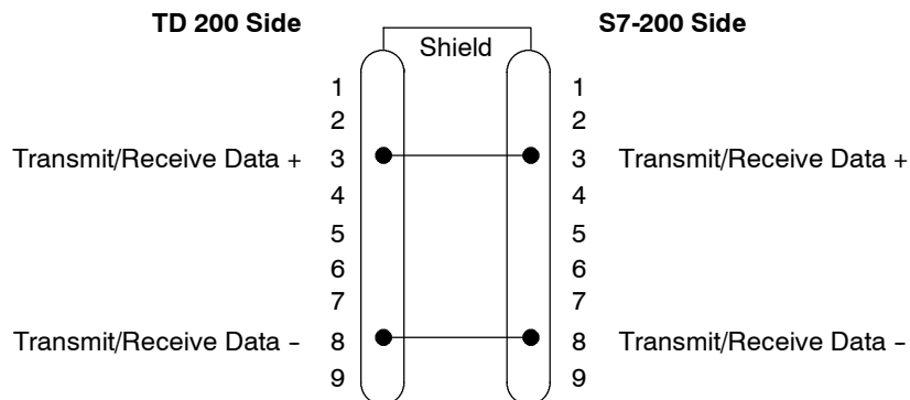
Figure B-5 TD/CPU Cable without Power Connections
