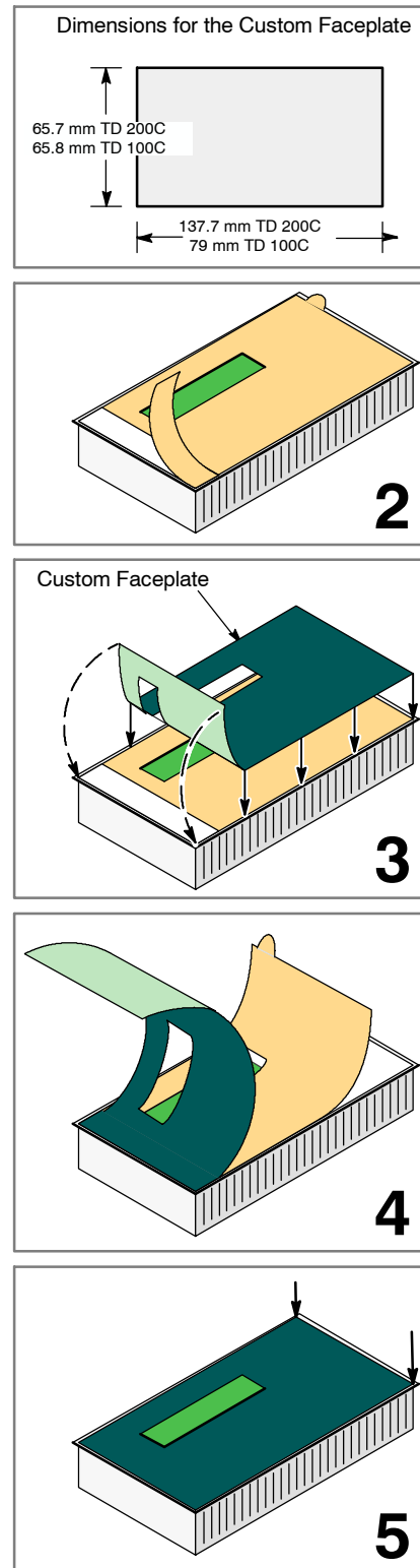
Figure 2-8 Installing a Custom Faceplate on a TD Device
