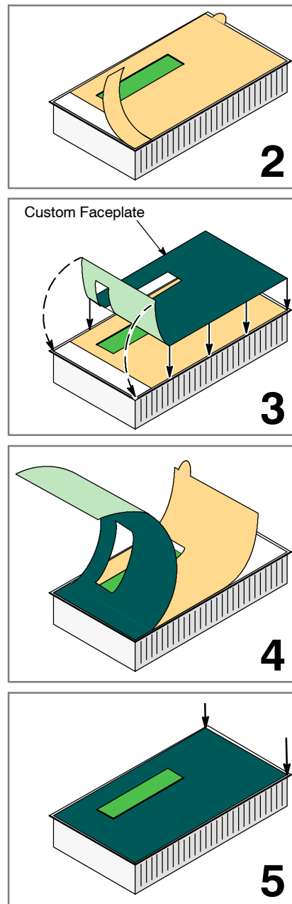
Figure 3-21 Adhering the Faceplate onto the TD Device
